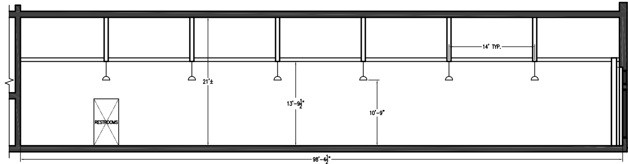
4 INTERIOR SOUTH WALL ELEVATION SCALE: 1/16" = 1'-0"
