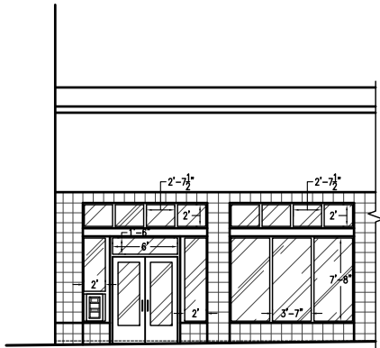
1 FRONT FACADE ELEVATION SCALE: 1/16" = 1'-0"
