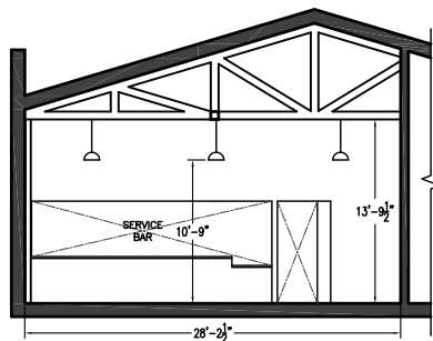
5 INTERIOR EAST WALL ELEVATION SCALE: 1/16" = 1'-0"
