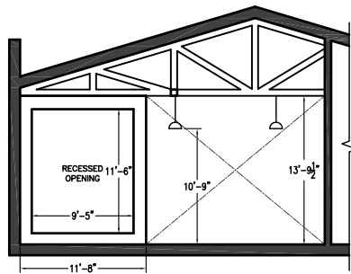
3 INTERIOR ENTRY WALL ELEVATION SCALE: 1/16" = 1'-0"
